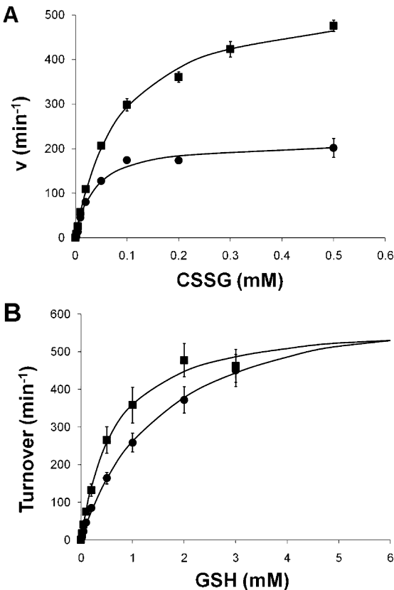
FIGURE 3: hGrx2 (C40S) exhibits higher K_{\text{M}} and V_{\text{max}} values for CSSG, but a lower K_{\text{M}} for GSH, than the wild-type enzyme does. Turnover of CSSG by wild-type [WT, 135 nM (●)] and C40S [135 nM (■)] hGrx2 was assessed via the spectrophotometric coupled assay (see Experimental Procedures) with a varied CSSG (0.002–0.5 mM) or GSH (0.02–3 mM) concentration, and velocity vs substrate curves were fit to the Michaelis–Menten equation. For wild-type hGrx2, apparent k_{\text{cat}} and K_{\text{M}} values for RSSG and GSH are listed in Table 2. For hGrx2 (C40S), k_{\text{cat,app,CSSG}} = 543 \pm 14 min -1 , K_{\text{M,app,CSSG}} = 0.083 \pm 0.009 mM, k_{\text{cat,app,GSH}} = 589 \pm 46 min -1 , and K_{\text{M,app,GSH}} = 0.63 \pm 0.1 mM. Each point represents the average of at least three determinations ± the standard error.
