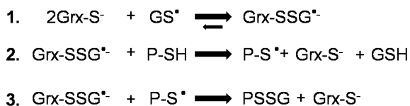
Scheme 3: Proposed Mechanism of GS • Transfer by Mammalian Grx1 (33) a
