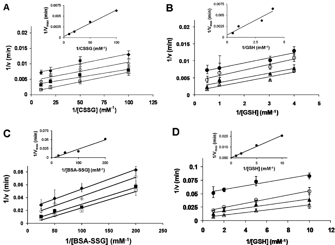
FIGURE 2: Two-substrate kinetic analysis of hGrx2-catalyzed deglutathionylation demonstrates a ping-pong kinetic pattern. The substrate dependence of Grx2-mediated reduction of R-SSG was determined using the standard spectrophotometric coupled assay (see Experimental Procedures). Reactions were initiated by addition of CSSG (for panels A and B) or GSH (for panels C and D). (A and B) Deglutathionylation of CSSG with or without hGrx2 in the presence of a fixed concentration of GSH with a varied CSSG concentration (A) or a fixed CSSG concentration and a varied GSH concentration (B): (A) (◆) 0.25 mM GSH, (◇) 0.3 mM GSH, (■) 1 mM GSH, and (□) 2 mM GSH and (B) (●) 0.01 mM CSSG, (○) 0.02 mM CSSG, (▲) 0.05 mM CSSG, and (△) 0.1 mM CSSG. (C and D) Deglutathionylation of BSA-SSG with or without hGrx2 in the presence of a fixed GSH concentration and a varied BSA-SSG concentration (C) or a fixed BSA-SSG concentration and a varied GSH concentration (D): (C) (◆) 0.1 mM GSH, (◇) 0.2 mM GSH, (■) 0.5 mM GSH, and (□) 1 mM GSH, and (D) (●) 5 \mu M BSA-SSG, (○) 10 \mu M BSA-SSG, (▲) 20 \mu M BSA-SSG, and (△) 40 \mu M BSA-SSG. Insets show secondary plots of the reciprocal of V_{\max} vs the reciprocal of RSSG concentration. V_{\max} values were calculated from fitting individual V vs [S] curves to the Michaelis-Menten equation. Data points represent the average of at least three experiments \pm the standard error, and when error bars are not visible, they are within the symbol.
