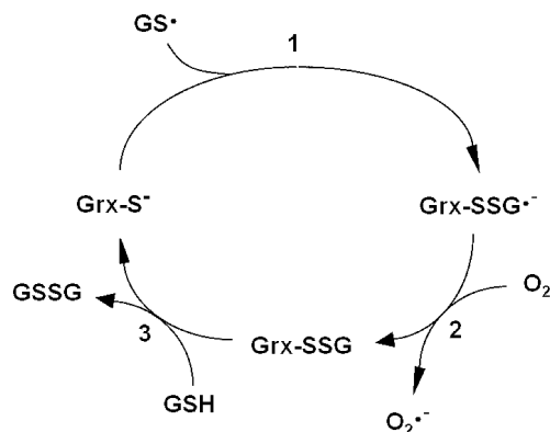
Scheme 2: Catalytic Mechanism of GS • Scavenging by Mammalian Grx1 (33) a
