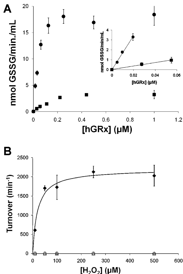
FIGURE 6: Thiyl radical ( \text{GS}^\bullet ) scavenging activity of Grx2. (A) hGrx (0–1 \mu\text{M} ) was preincubated with 0.5 mM GSH, 0.2 mM NADPH, and 2 units/mL GSSG reductase in 0.1 M Na/K phosphate buffer (pH 7.5) at 30 °C for 5 min (see Experimental Procedures and ref 33). Then a premade complex containing \text{FeCl}_2 (0.5 mM) and ADP (2.5 mM) was added to each, and the reactions were initiated by addition of \text{H}_2\text{O}_2 (50 \mu\text{M} ). Reactions were monitored according to the decrease in A_{340} over 5 min (within the linear range of time dependence). The amount of GSSG formed per minute was calculated according to the extinction coefficient of NADPH, corrected for the plate reader assay (see Experimental Procedures). The inset shows a region of linear dependence on hGrx concentration. GS radical scavenging activities in this time period were used to calculate turnover [hGrx1 (●), 170.0 \pm 7.7 ; hGrx2 (■), 18.7 \pm 1.2 ; 9.1 hGrx1:hGrx2 ratio]. Symbols represent the means of four to six determinations \pm the standard error. (B) GSH-dependent peroxidase activity was measured in 0.1 M Na/K phosphate buffer (pH 7.5) containing GSH (0.5 mM) and GSSG reductase (2 units/mL). Reactions were initiated by addition of \text{H}_2\text{O}_2 , and A_{340} was monitored over 5 min. Rates of GSSG formation (i.e., NADPH oxidation) were calculated using the extinction coefficient of NADPH. Glutathione peroxidase (GPx) was used as a positive control: (◆) GPx (5 nM), (○) hGrx1 (1 \mu\text{M} ), and (△) hGrx2 (1 \mu\text{M} ). Each symbol represents the average of at least three determinations \pm the standard error. When error bars are not visible, they are within the symbol.
