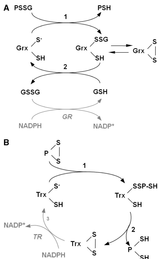
Scheme 1: (A) Catalytic Mechanism of Protein Deglutathionylation by Mammalian Grx1 (16, 18) and Grx2 and (B) Catalytic Mechanism of Intramolecular Disulfide Reduction by Mammalian Trx (5, 57) a
