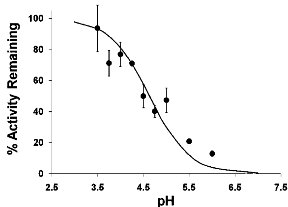
FIGURE 5: Determination of the pK_a of the active site Cys-SH of hGrx2. hGrx2 (3 \mu\text{M} ) was incubated with iodoacetamide (IAM, 0.3 mM) for 3 min in the following incubation buffers: sodium citrate at pH 3.5; sodium acetate at pH 3.5, 4.0, 4.5, and 5.0; and 2-( N -morpholino)ethanesulfonic acid (MES) at pH 5.0, 5.5, and 6.0. All buffers were at a concentration of 10 mM, and the ionic strength was adjusted to 0.5 M by addition of the appropriate amount of NaCl or KCl. Following incubation, hGrx2 activity was determined using the standard spectrophotometric coupled assay (Experimental Procedures) after a 50-fold dilution into the assay mix [0.1 M Na/K phosphate (pH 7.5), 0.2 mM NADPH, 0.5 mM GSH, and 2 units/mL GSSG reductase]. The percent activity remaining at each pH was determined from the ratio of Grx2-mediated deglutathionylation rates for enzyme preincubated with IAM versus no IAM (see Experimental Procedures). Symbols represent the mean of at least three determinations of hGrx1 activity with or without IAM preincubation \pm the standard error. When error bars are not visible, they are within the symbol.
